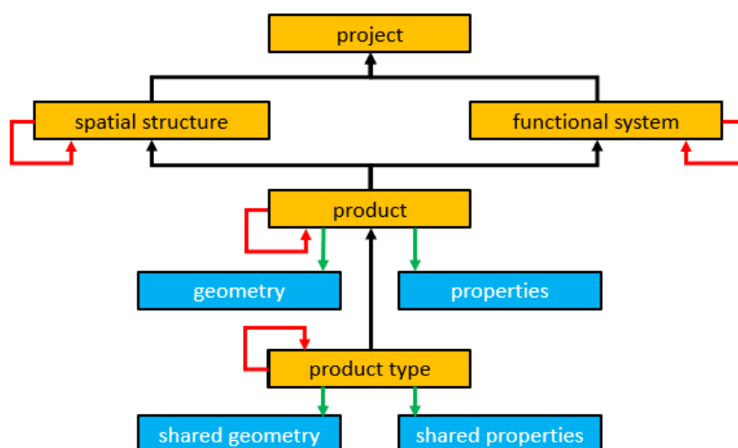
Figure 2: Conceptual Model of IFC Tunnel (simplified view)
