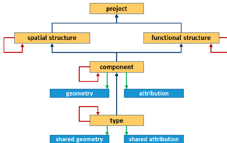
Figure 4: Extract from IFC Infra Overall Architecture Project - Documentation and Guidelines – buildingSMART International, 2016
